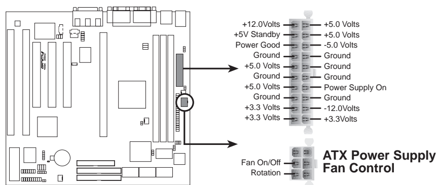
P2L-VM/P2E-VM ATX Power Connector
